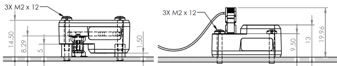
Figure 7: Connection options (left: PCB, right: standalone, dimensions in mm)
