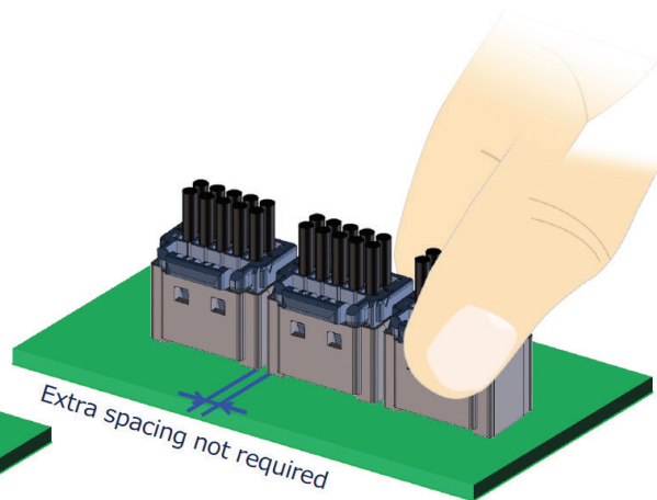
Center-Lock Type (DF51K)
