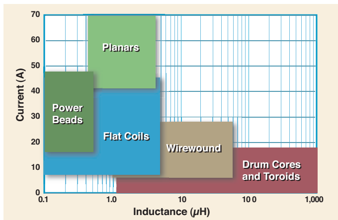
Fig. 1 Current and inductance characteristics of the various types of power inductors.
