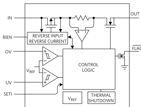
Figure 8. Integrated protection in a single IC.
