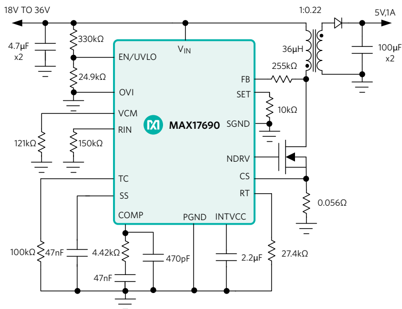
Figure 6. No-opto flyback controller.
