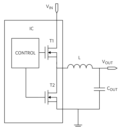
Figure 4. Fully integrated synchronous buck converter.
