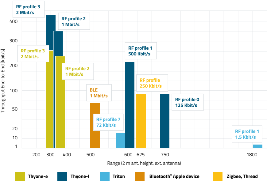
Comparison 2.4 GHz modules Thyone-I, Thyone-e and Triton
