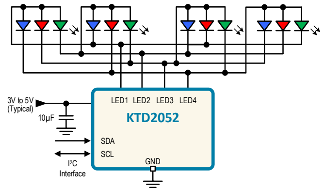
12-Channel RGB LED Driver with I²C Control
