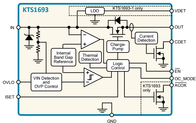
20V/6A, \pm 100V Surge, 5.95V Fixed or Adjustable OVP with adj. OCP
