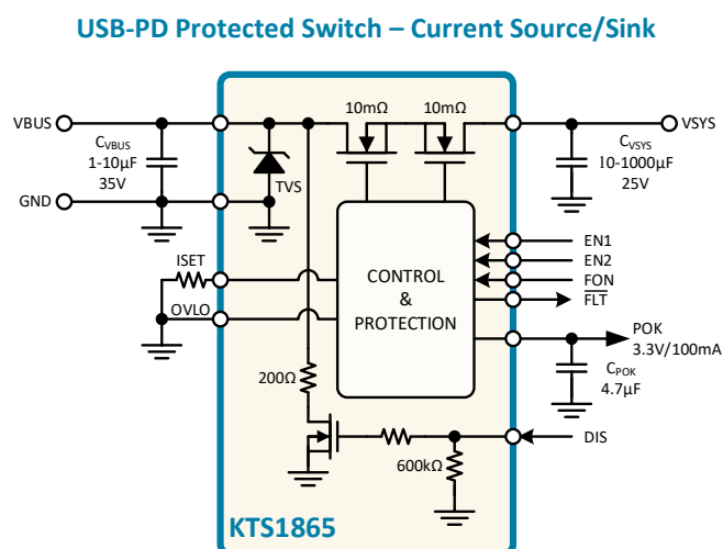
20V/6.5A, \pm 100V Surge, Bi-Directional Load Switch with OVP, OCP, RBP, RCP, CL, SCP and POK Safe LDO
