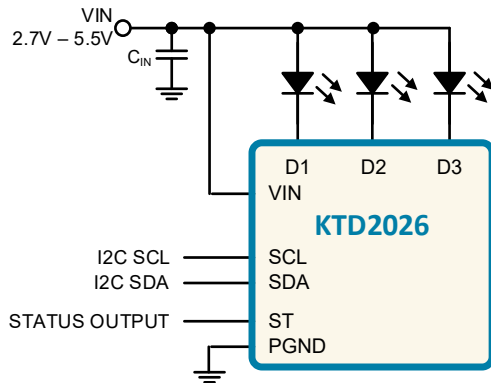
3-Channel RGB LED Driver with I²C Dimming
