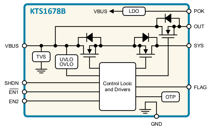
Single Input, Dual Output, 20V, 3.5A/6A, \pm 100V Surge, 13.9V/5.25V Fixed OVP with RBP
