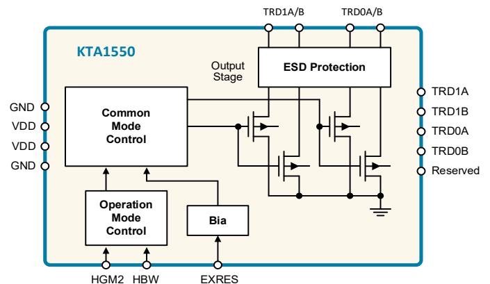
Dual Channel Active EMI & ESD Suppressor
