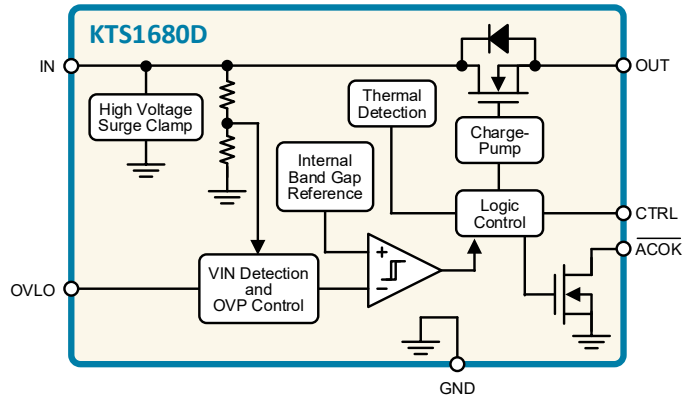
20V/4.5A, 13.9V Fixed or Adjustable OVP with \pm 100V Surge Protection
