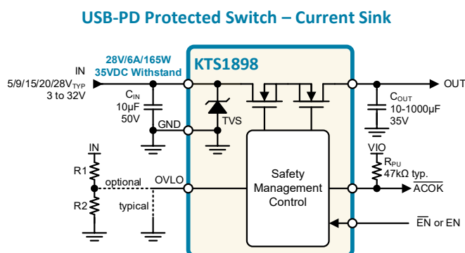
6.5A, \pm 100\text{V} Surge, 35V OVP Switch with RBP, RCP and SCP
