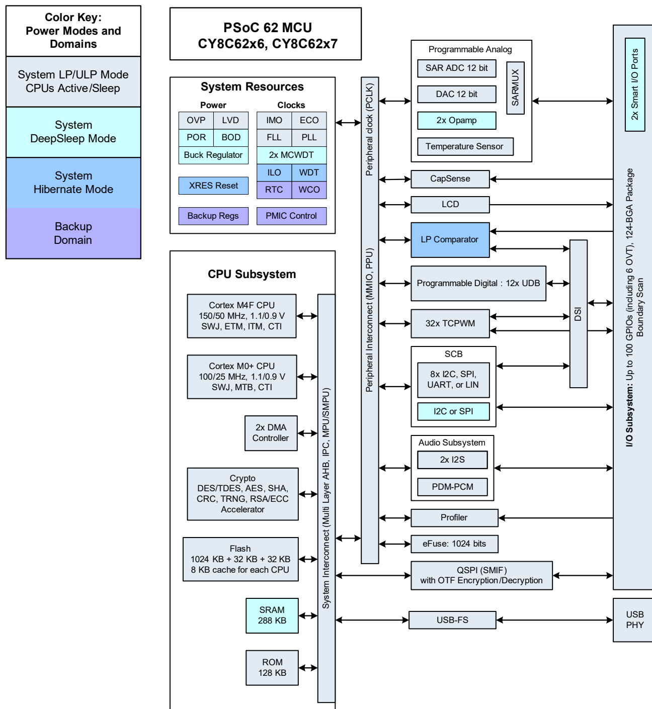
Figure 3. Block Diagram
