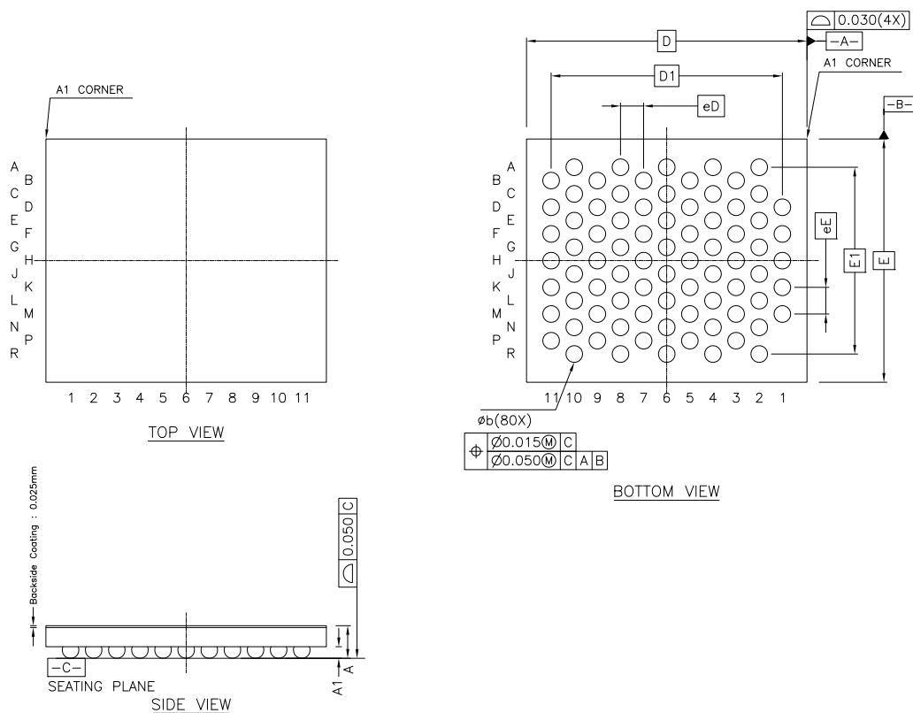
Figure 14. 80-Ball WLCSP 3.676 × 3.190 × 0.467 mm
