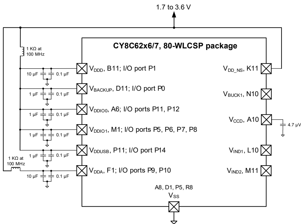
Figure 11. 80-WLCSP (No Buck) Power Connection Diagram
