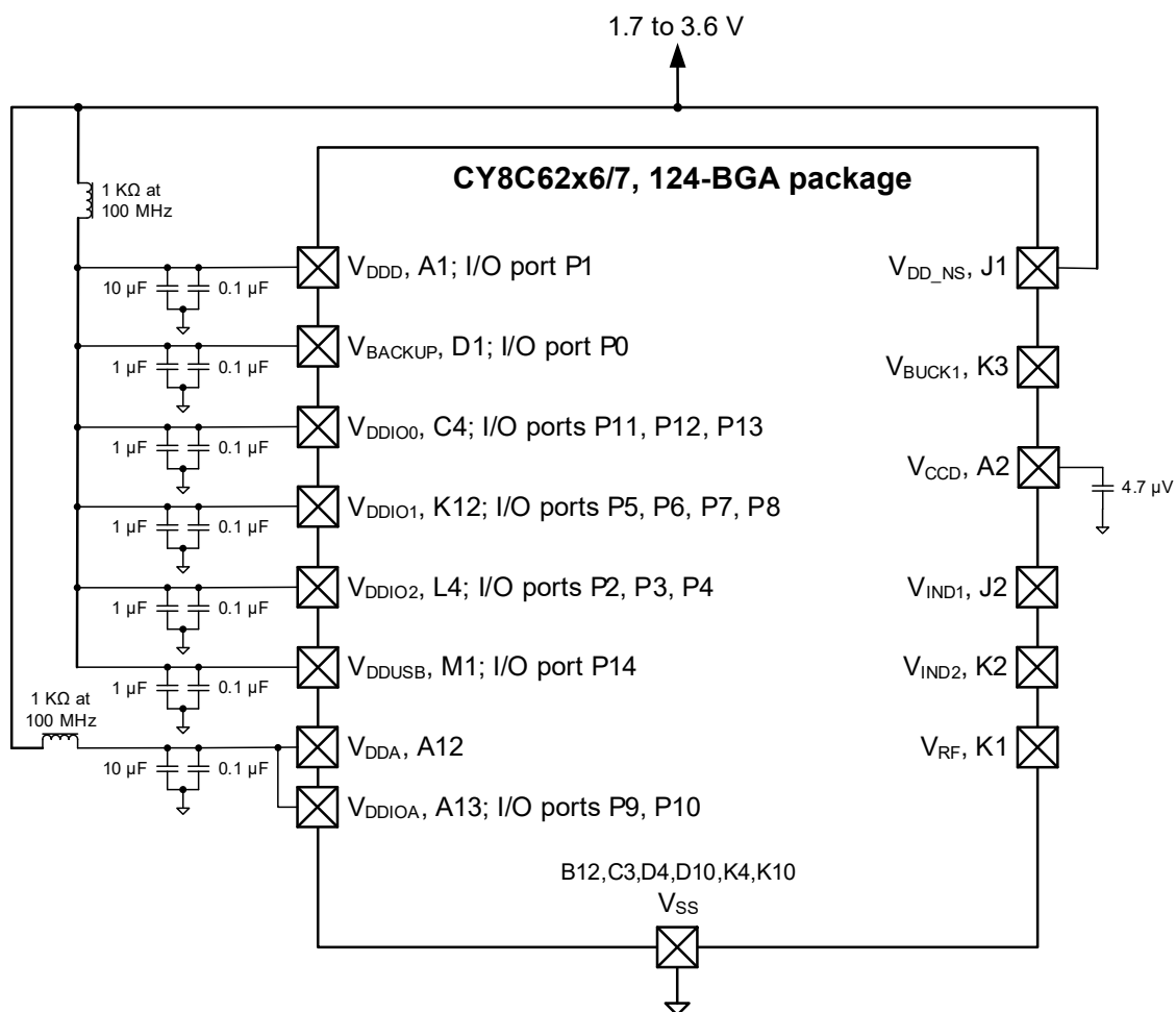
Figure 9. 124-BGA (No Buck) Power Connection Diagram
