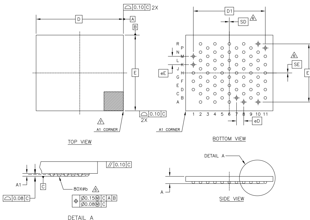
Figure 15. Thin 80-Ball WLCSP 3.676 × 3.190 × 0.33 mm
