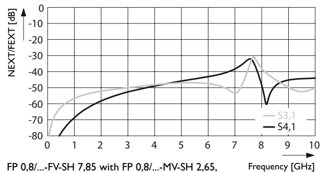
FP 0,8/...-FV-SH 7,85 with FP 0,8/...-MV-SH 2,65, differential pair, 12 mm stack height
