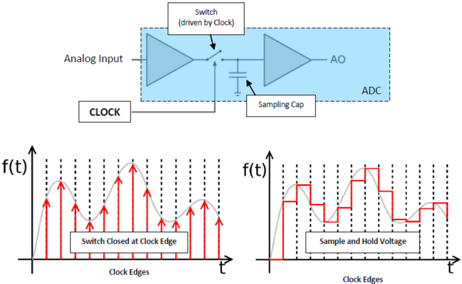
Figure 10. Sample &amp; Hold Circuit (ADC Use Case)
